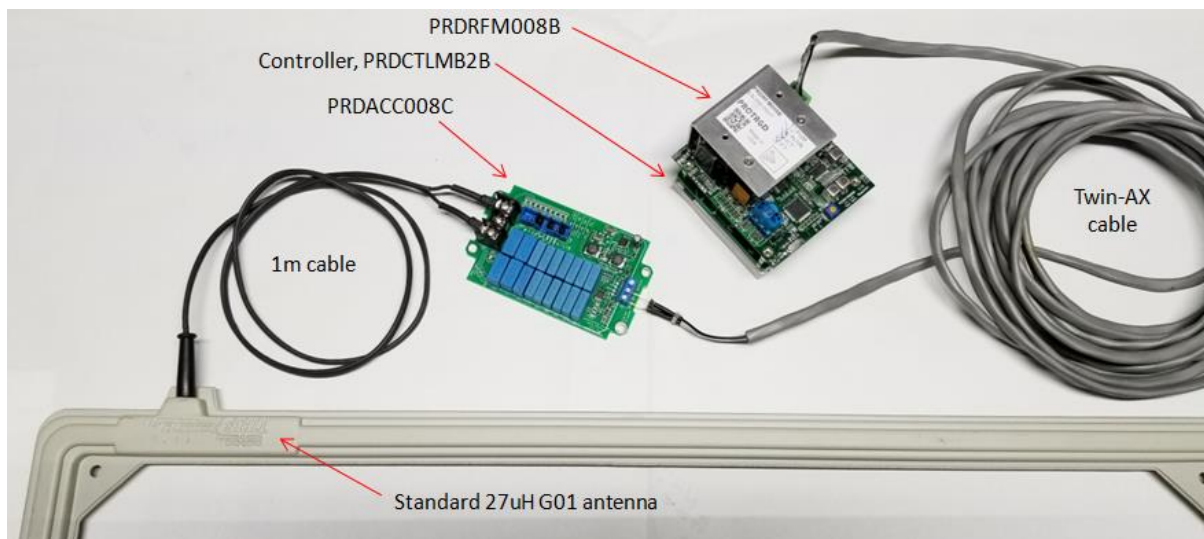
Figure 5.1 Connections
